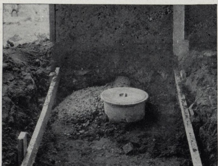
Water pipes for individual drinking cups and drains in gutter and mangers must be installed before placing the concrete
