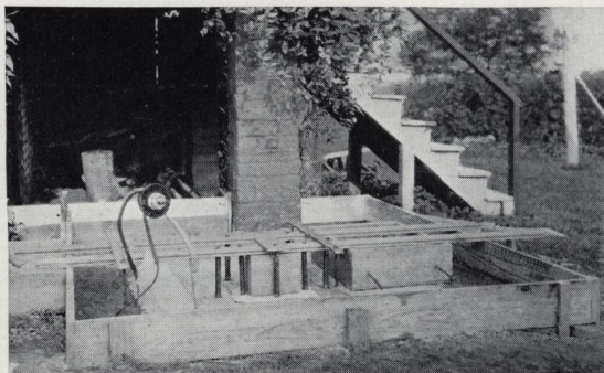
Concrete well cover, with electrically operated pump jack, enclosed in a shed for protection against weather. The illustration above shows the forms ready to receive the concrete
