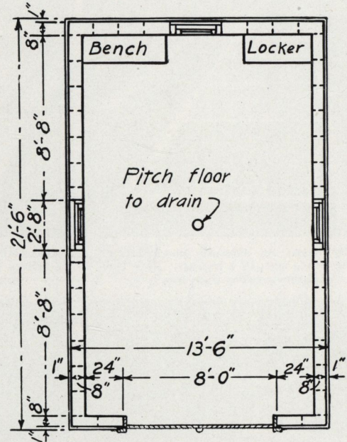
Plan of concrete block garage
