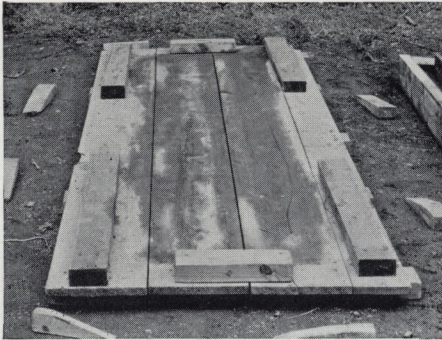
Forms for fence posts are easily made. The mold illustrated here will cast four posts. The platform is 3 feet wide by 8 feet long
