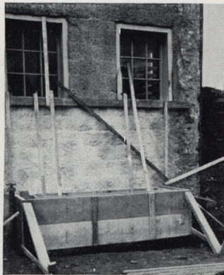
A 1:2:3 mixture will give water-tight concrete provided it is well tamped while being poured
