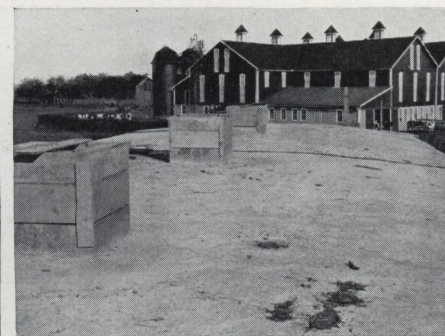
Roof completed. The three forms in the center of the roof are for the construction of the concrete ventilators
