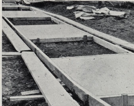
Alternate blocks are poured, using a 1: 2½: 4 concrete mixture (1 part cement, 2½ parts sand and 4 parts stone or gravel)
