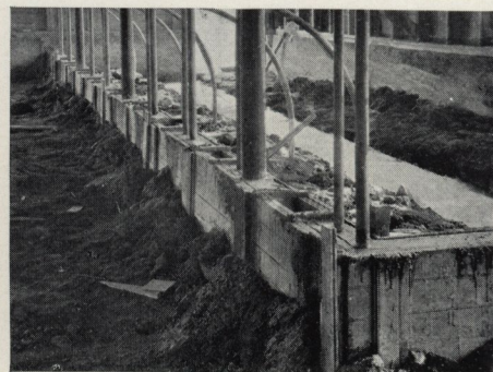
The curb between the manger and the stall is poured first, to hold the steel stall posts in place. Remove sharp corners with an edger
