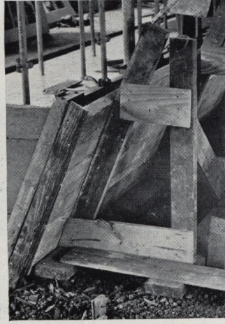
The forms must be well braced to support the weight of the wet concrete
