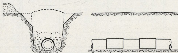
Drain tile laid in trench. Tar paper placed over joints. Surround with gravel, and fill trench with soil
