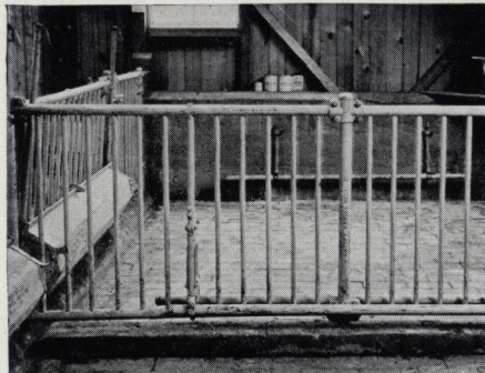
Metal partitions erected. Posts are placed in holes formed by anchors, and a 1:3 concrete mixture poured around them
