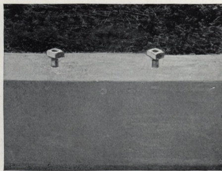
Forms removed from curb, showing bolts in the concrete ready to receive the dairy barn equipment
