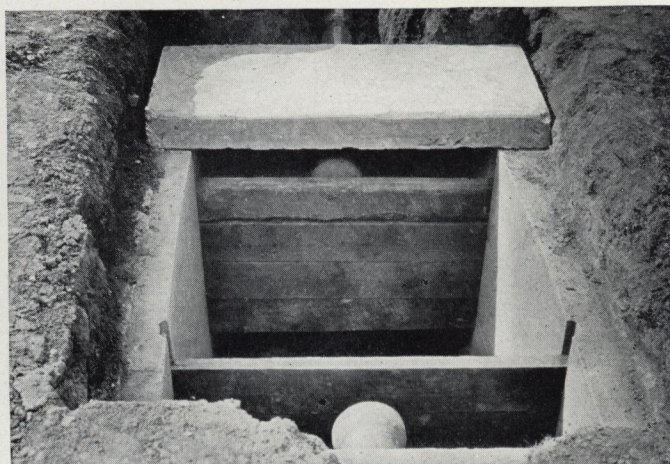
One of the cover sections in place. It is not necessary to seal the joints between the cover slabs, as the earth covering will aid in keeping the tank sufficiently air tight
