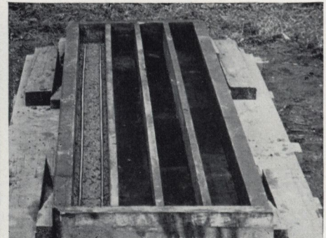
Place a one-inch layer of concrete in the molds. Tamp thoroughly. Put in two ¼" rods for reinforcement
