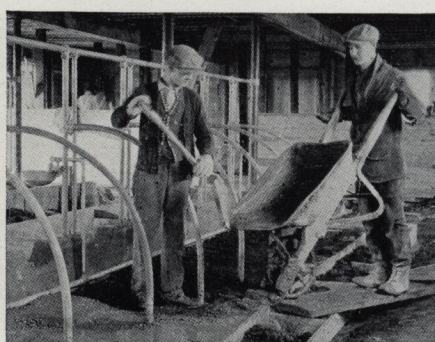
Placing the concrete for the stall floor. This floor should be from 2 to 4 inches above the level of the litter alley
