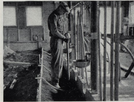
Form is partially filled with earth, tamped thoroughly to provide a solid foundation. Leave room for a 4-inch layer of concrete
