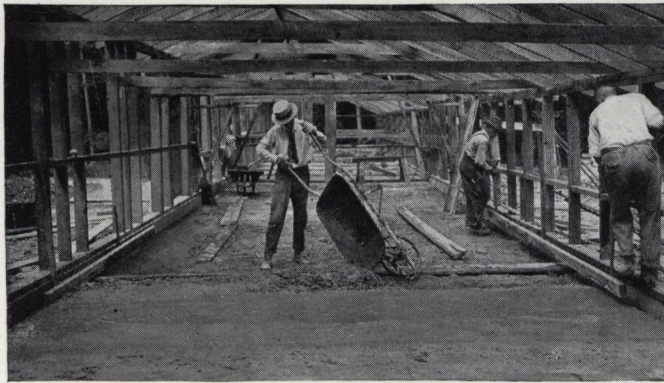
Pouring a 4-inch layer of concrete for the floor. Tamp thoroughly to make a dense, solid mass. The two men at the right are placing a 2 x 4 at the correct floor level
