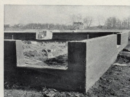
Forms removed. The wall is now ready for the superstructure. Note the bolts for anchoring sill to the foundation
