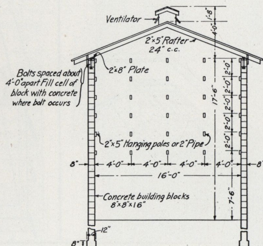
Cross-section
