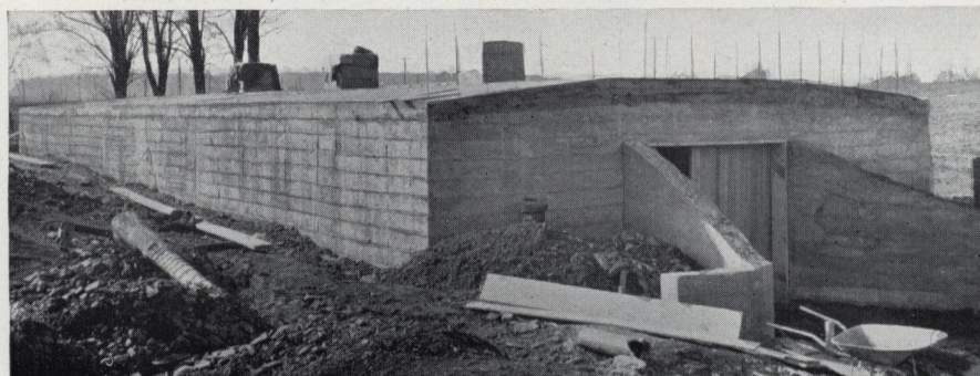
Storage cellar practically completed, ready to be covered with earth. For storage purposes, wall types A, B and C, illustrated on page 12, will serve as satisfactorily as the hollow wall (type "D") shown here
