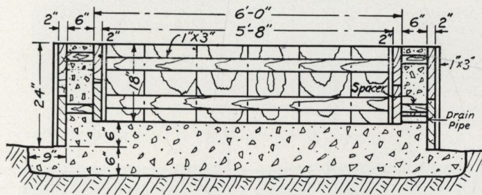
Cross-section lengthwise
