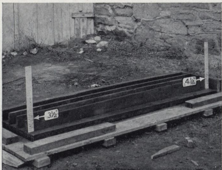
The difference of ¾ inch in the width of these strips tapers the posts. One end will be 4¼ inches wide; the other, 3½ inches
