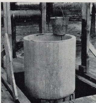
The large sizes of concrete pipe make an excellent lining as an alternative for poured concrete
