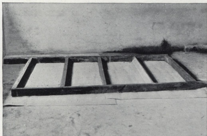
Forms for cover slabs are made of 2 x 4 inch lumber. Four sections are advisable because of the weight in handling. Note that one section is beveled to permit easy removal when cleaning tank
