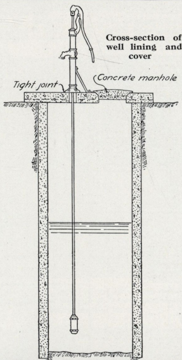
The large sizes of concrete pipe make an excellent lining as an alternative for poured concrete
