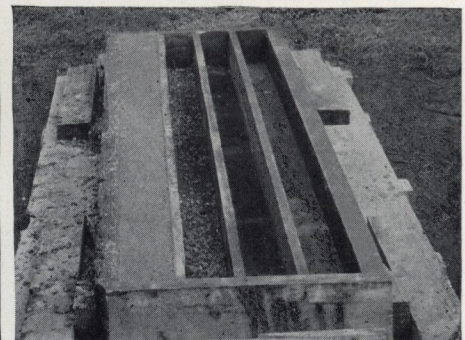
Fill mold with concrete. Thorough tamping is necessary to obtain good posts. Finish with a steel trowel
