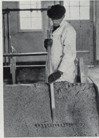
A thin layer of 1:3 concrete (one part cement and three parts sand) is now placed
