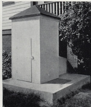
Concrete well cover, with electrically operated pump jack, enclosed in a shed for protection against weather. The illustration above shows the forms ready to receive the concrete
