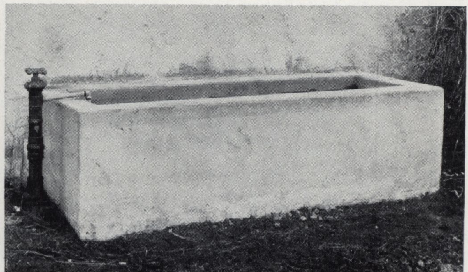
Remove inside forms in 24 hours and fill tank with water. Remove outside forms in one week. To remove the marks of the wooden forms, rub with an abrasive stone as soon as forms are off
