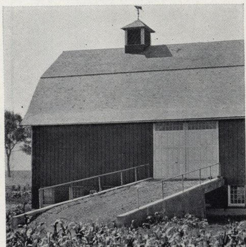
A concrete barn approach is a worthwhile improvement. It keeps the soil in place during heavy rains and the concrete walls present a neat and attractive appearance
