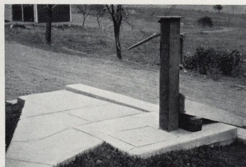
A 1:2:3 mix should be used for linings, as a water-tight wall is necessary. A 1:2:4 mix is satisfactory for the reinforced cover slab
