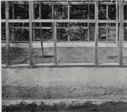
The foundation wall for a poultry house, with sills and framing in position. Foundation should extend below the frost line
