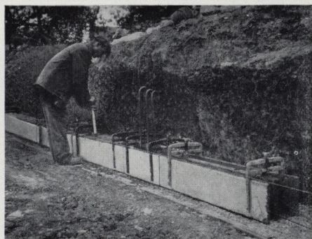
Hollow-wall molds are needed to cast the type "D" wall (see page 12 for detailed drawing) for a concrete storage cellar
