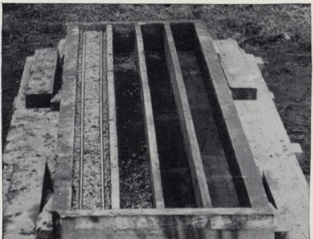
Fill mold with concrete to within 1 inch of top. Tamp concrete again. Place two more reinforcing rods in position
