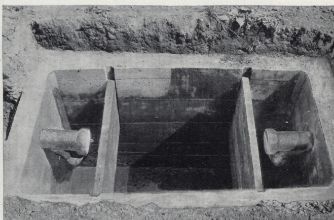
The baffle-boards, made of 2-inch planks, preferably of cypress or chestnut, can now be put in place and wedged tight. These baffles prevent a direct current from inlet to outlet
