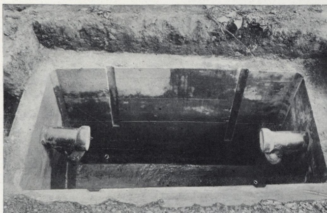
Allow concrete to harden from five to seven days before removing forms. First remove center brace, then draw nails holding the 2 x 4 corners to the sides. Remove ends of forms, then the sides
