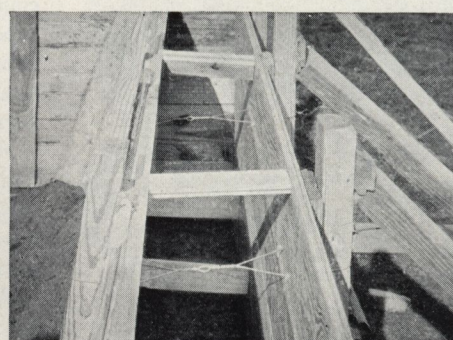
Tie-wires and spreaders. Wires are twisted until forms are tight. Spreaders are removed before concrete covers them
