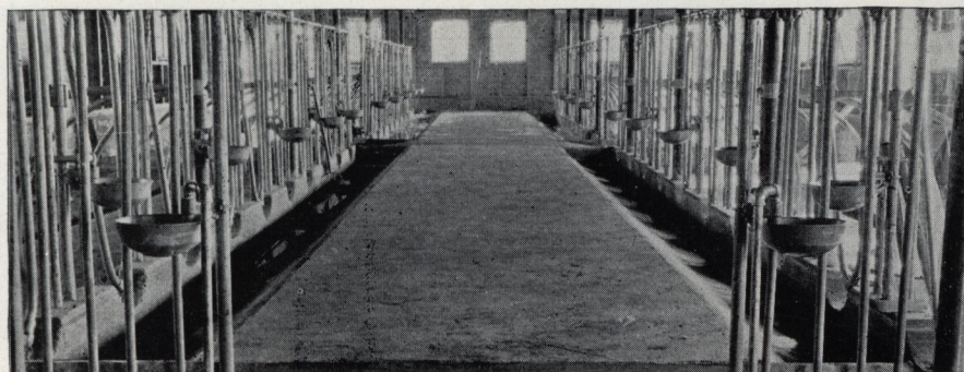
The concrete for the feed alley can now be placed between the mangers, after filling in with well-tamped earth to the required level. This installation shows a feed alley raised to the top of the mangers. Another type is illustrated on page 7
