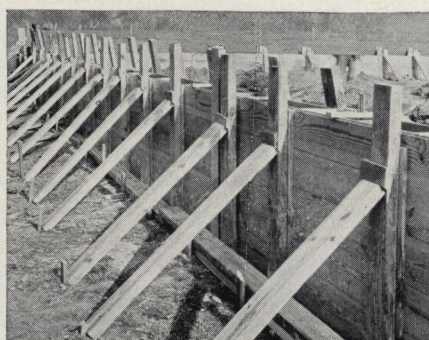
Method of bracing side wall. Use but few nails. Practically all this form lumber can later be used in the building
