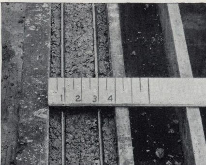
Place reinforcing about 1 inch from the outside of posts. If placed nearer the edge, rods will rust and concrete will break
