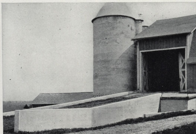
Reinforced suspended slab with \frac{3}{8} inch bars spaced 10 inches from center to center, placed 1\frac{1}{2} inches from the bottom of the slab. Spans larger than 8 feet should be computed by an engineer
