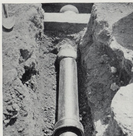
Inlet line joining Y-branch. There is no bell at the tank joint, and a band of concrete is placed around the ends of pipe
