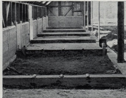
Forms for concrete curbing to hold metal partitions between the pens. In rear, floors have been poured
