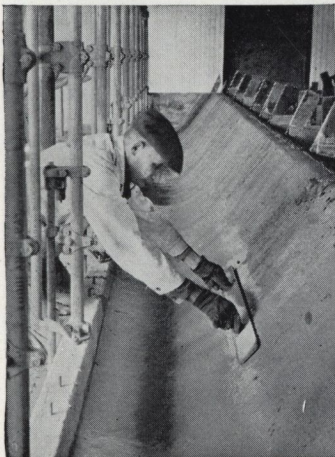
The final finishing coat is a very thin layer of one part cement and three parts fine sand
