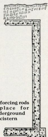
Showing placement of reinforcing rods for retaining wall
