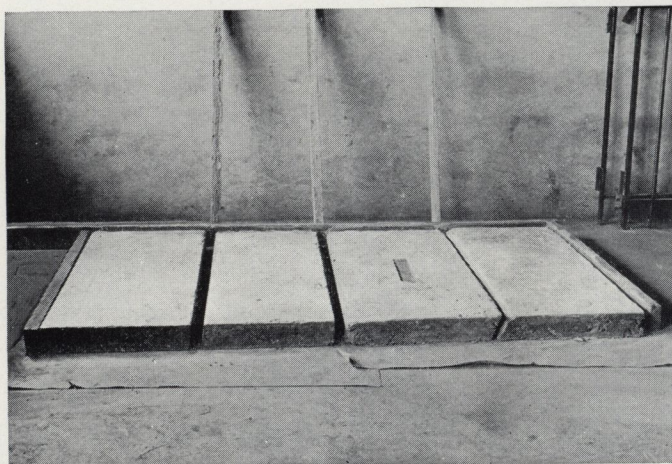
Forms removed from cover slabs. The beveled section has been marked "I" to identify it when it is necessary to lift covers to clean tank. This section can then be lifted off first
