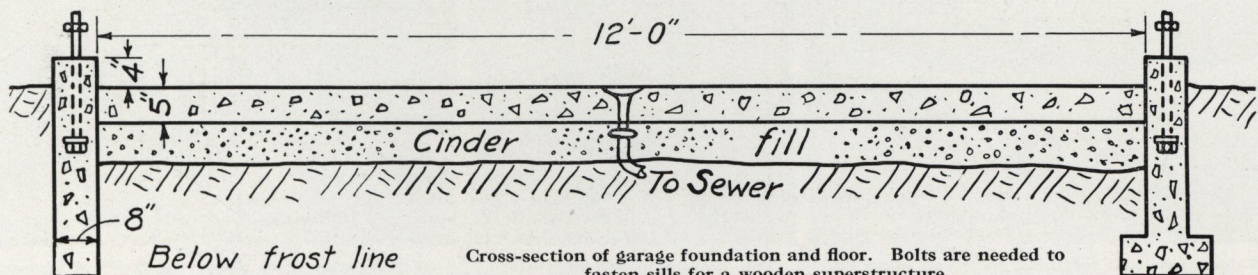
Concrete garage floor
