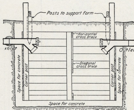
Forms in place, supported by cross-arms
