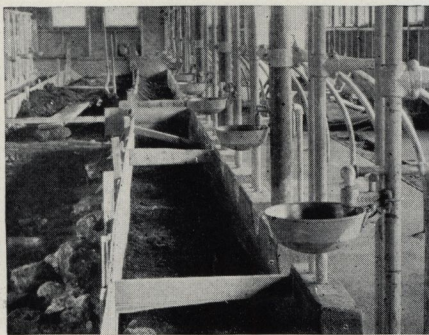
Forms for feed manger. Steel templets, placed 3 to 4 feet apart, to form the curve, are shown in next illustration
