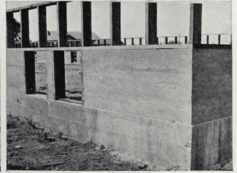
Detail of corner of concrete wall. Note the doors in the wall for entrance between pens and outside runs
