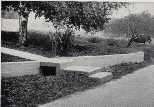
Walks, steps and retaining walls can often be combined in a practical and pleasing manner
