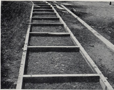
Sturdy forms for sidewalk construction can be made with 2 x 4 lumber. Note the division between each block
