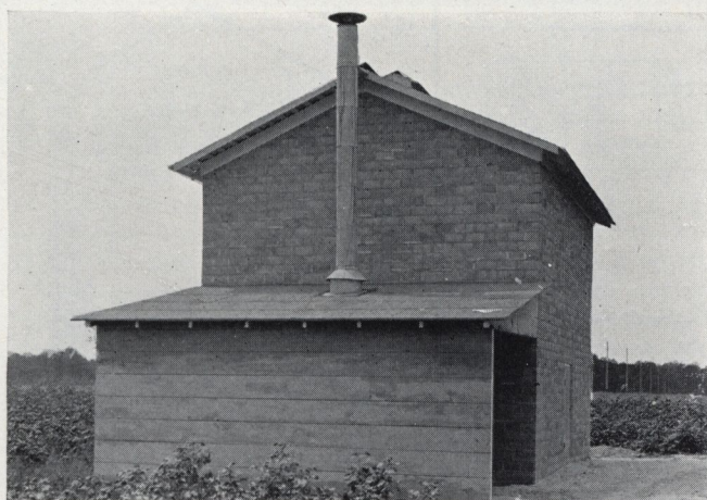
View from furnace end of building. A shed has been erected for convenience in tending the fire in wet weather
