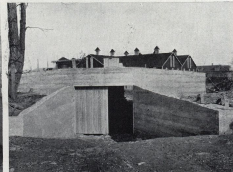
Wing walls solid concrete, 10" thick. Carry footings below frost line. Reinforcing rods should be used where wall joins cellar
