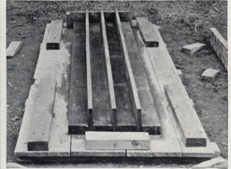
For separators between posts, strips of one-inch lumber, 5½ to 6¼ inches wide, are stood on edge
