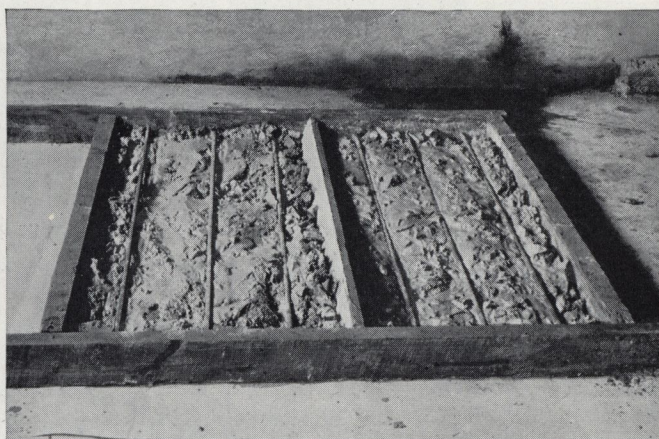
Fill forms with a mixture of 1:2:3 concrete. Reinforcement of half-inch bars or of expanded metal lath should be placed \frac{3}{4} inch from the under side of the slab
