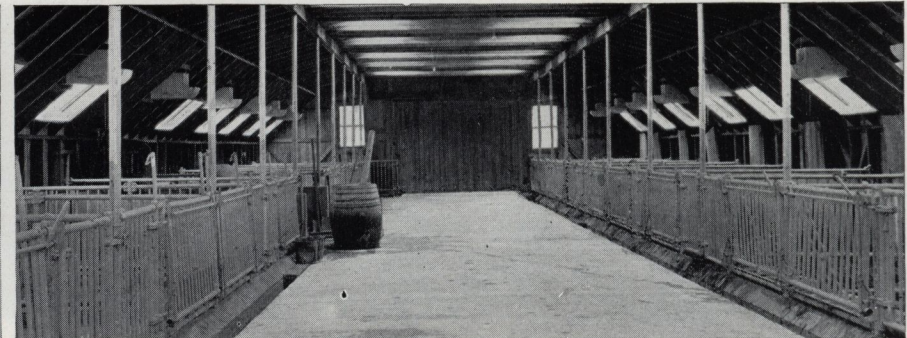
Interior view of completed hog house. It is warm and dry, and there is an abundance of direct sunlight. The concrete construction offers superior sanitary advantages. Smooth walls and floors, with no inaccessible crevices, encourage healthfulness
