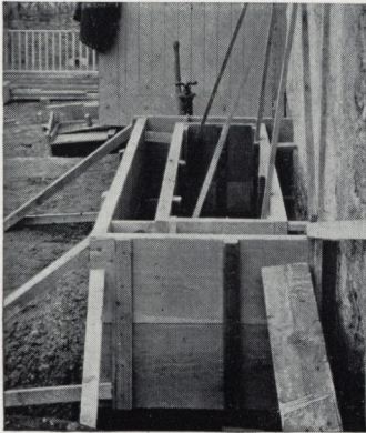
Forms for concrete water trough have been suspended from above and braced against the wall.
