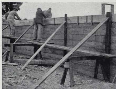
Forms to hold the concrete for the roof slab are being built. They should be braced firmly against the side wall
