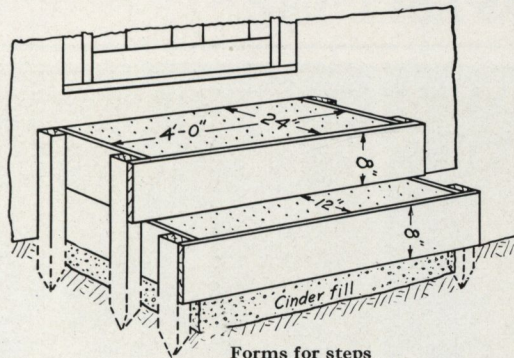
Forms for steps
